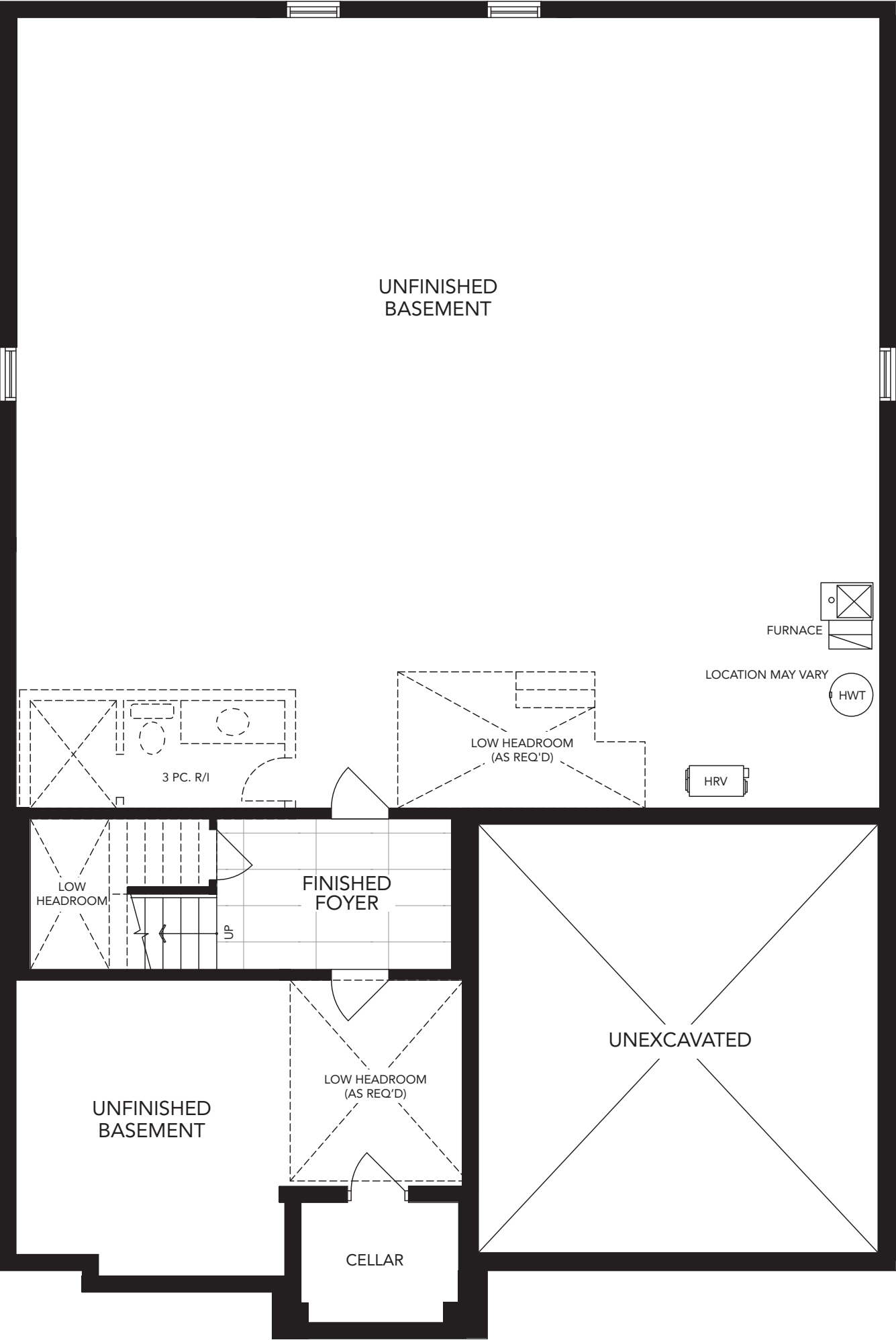
Basement Floor Plan Elevation A
