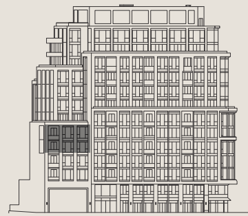
NORTH VIEW
