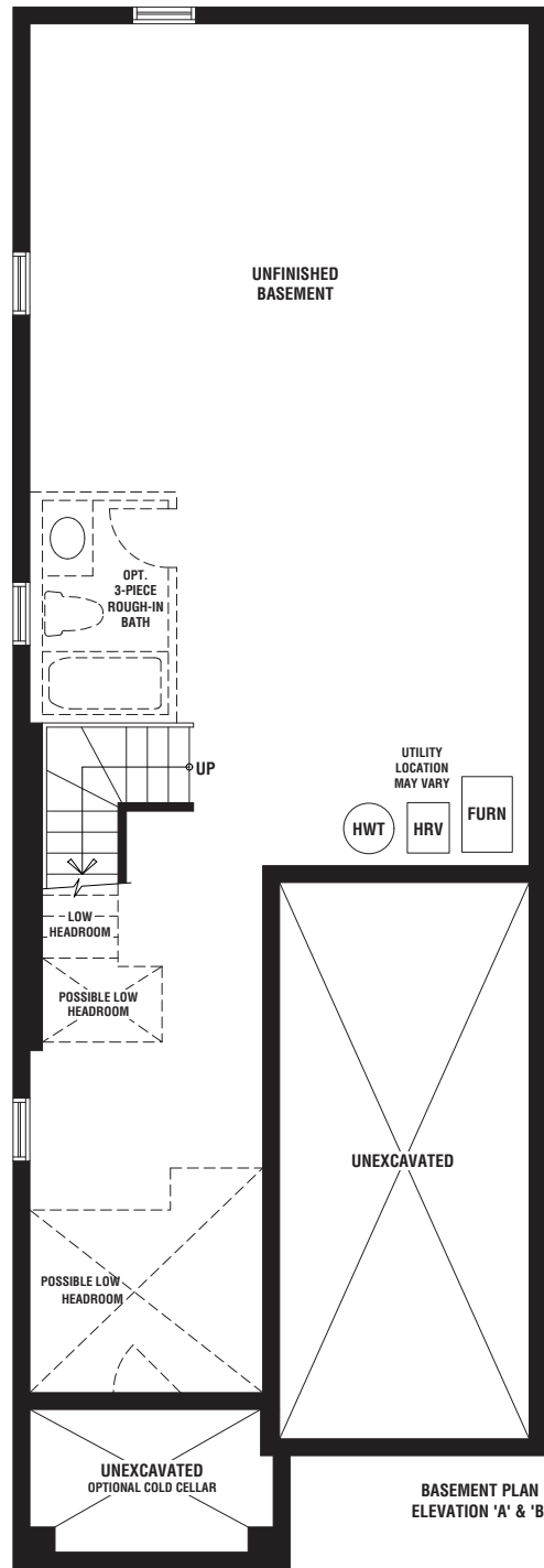
PARTIAL BASEMENT PLAN FOR OPTIONAL GROUND FLOOR PLAN ELEVATION 'A' & 'B'
