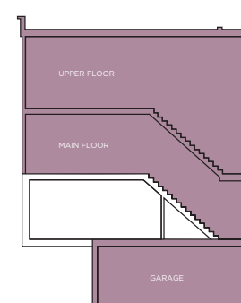
SIDE ELEVATION
