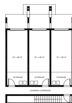
GARAGE PLAN
