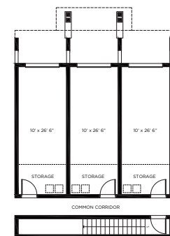
GARAGE PLAN
