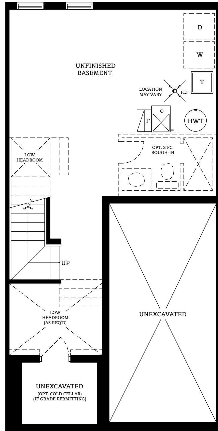
BASEMENT PLAN ELEV. 'C'
