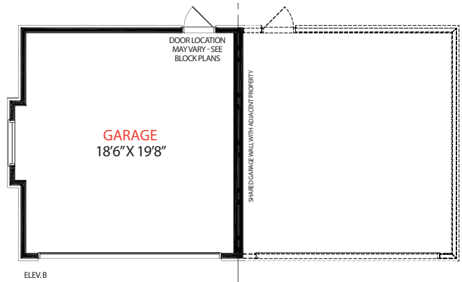
SEMI-DETACHED LANEWAY (SIDE UPGRADE)
