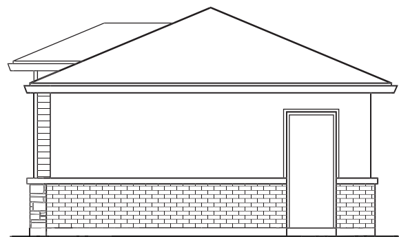
ELEV. B DOOR LOCATION MAY VARY - SEE BLOCK PLANS DETACHED (SIDE UPGRADE) REAR
