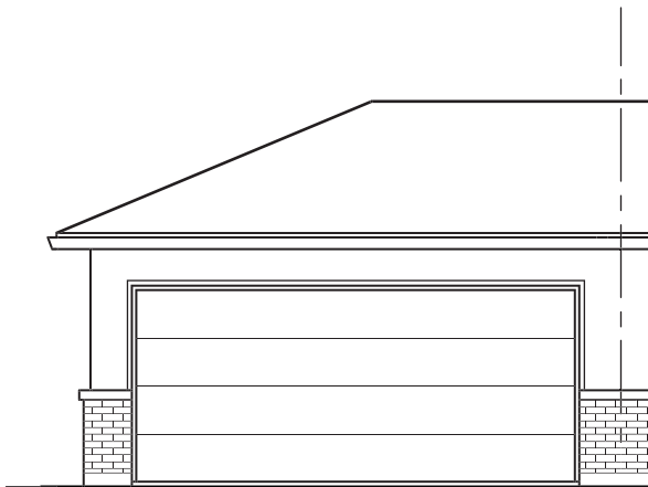
SEMI-DETACHED LANEWAY
