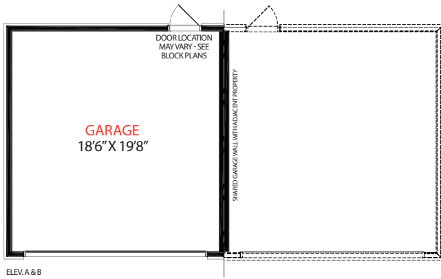
SEMI-DETACHED LANEWAY
