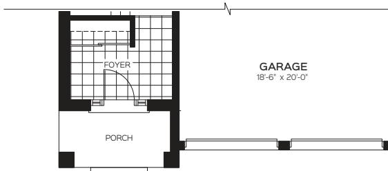
PARTIAL GROUND FLOOR ELEV. B
