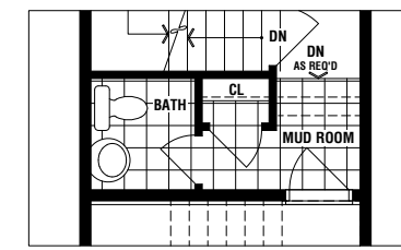
PARTIAL OPTIONAL BATH LAYOUT ELEVATION 'B' SIMILAR)
