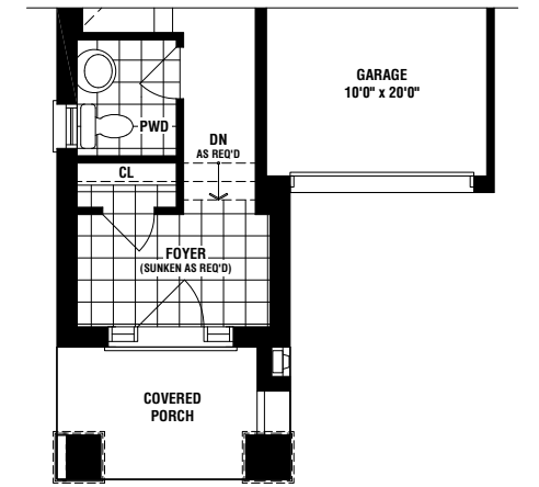
PARTIAL GROUND ELEV. 'B'
