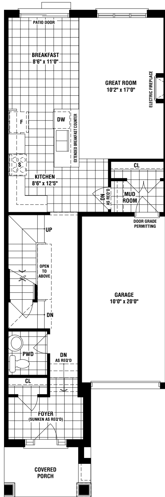
GROUND FLOOR ELEV. 'A'
