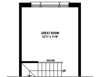
PARTIAL MAIN FLOOR ELEV. 'B'
