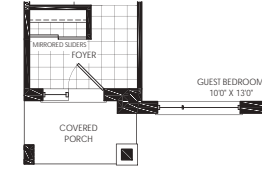
PARTIAL LOWER FLOOR STYLE 'B1'
