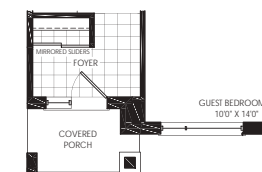
PARTIAL LOWER FLOOR STYLE 'B2'
