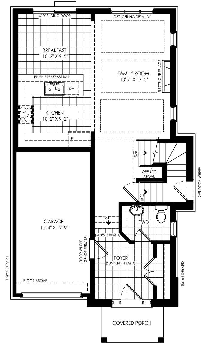
GROUND FLOOR PLAN ELEVATION 'F'
