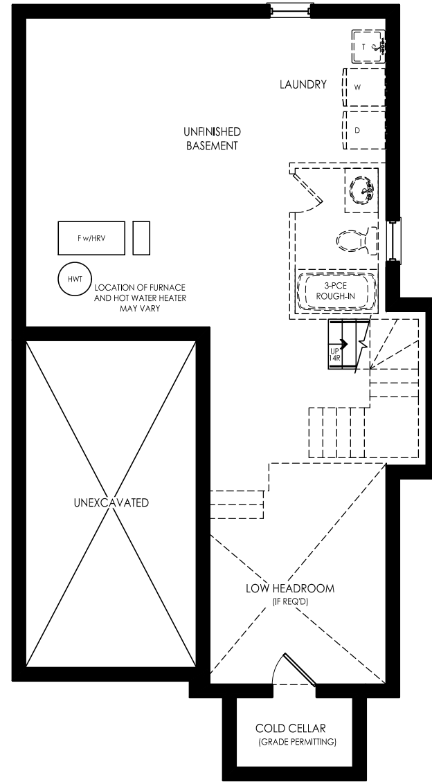
BASEMENT PLAN ELEVATION 'F'
