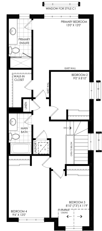
ALT. 4 BEDROOM UPPER FLOOR STYLE 'B1' & 'B2'
