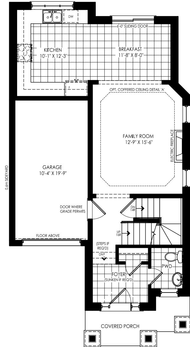
MAIN FLOOR PLAN ELEVATION 'T'
