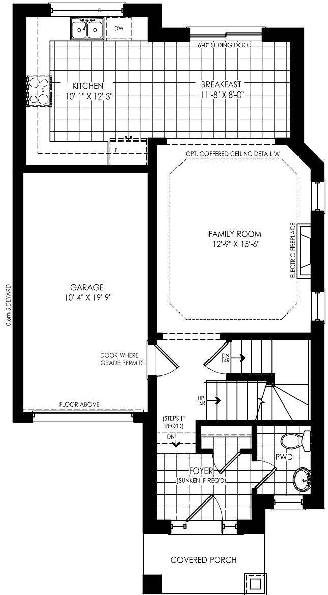
MAIN FLOOR PLAN ELEVATION 'C'
