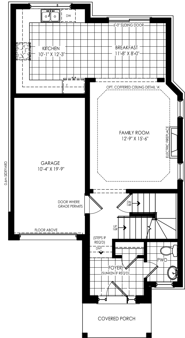
MAIN FLOOR PLAN ELEVATION 'F'
