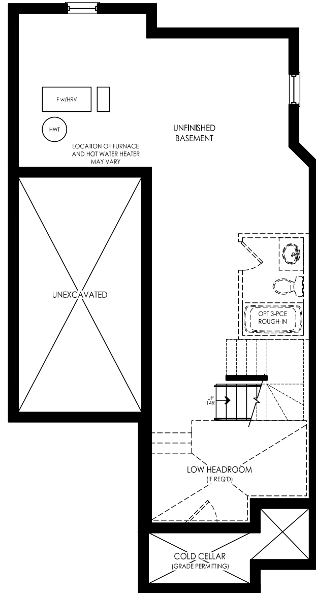
BASEMENT PLAN ELEVATION 'T'
