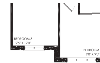
PARTIAL SECOND FLOOR STYLE 'B2'
