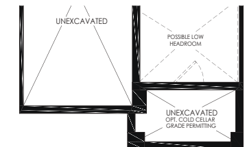
PARTIAL BASEMENT FLOOR STYLE 'C1'
