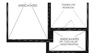
PARTIAL BASEMENT FLOOR STYLE 'B2'
