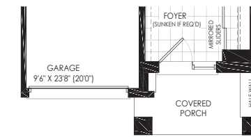
PARTIAL GROUND FLOOR STYLE 'C1'
