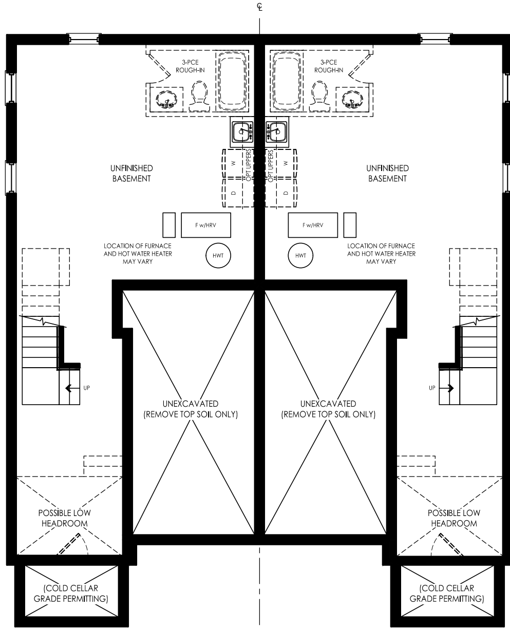
BASEMENT PLAN ELEVATION 'F-1'
