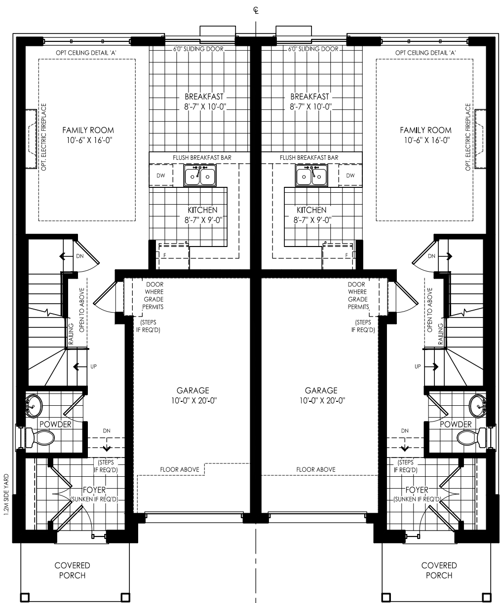
MAIN FLOOR PLAN ELEVATION 'F-1'
